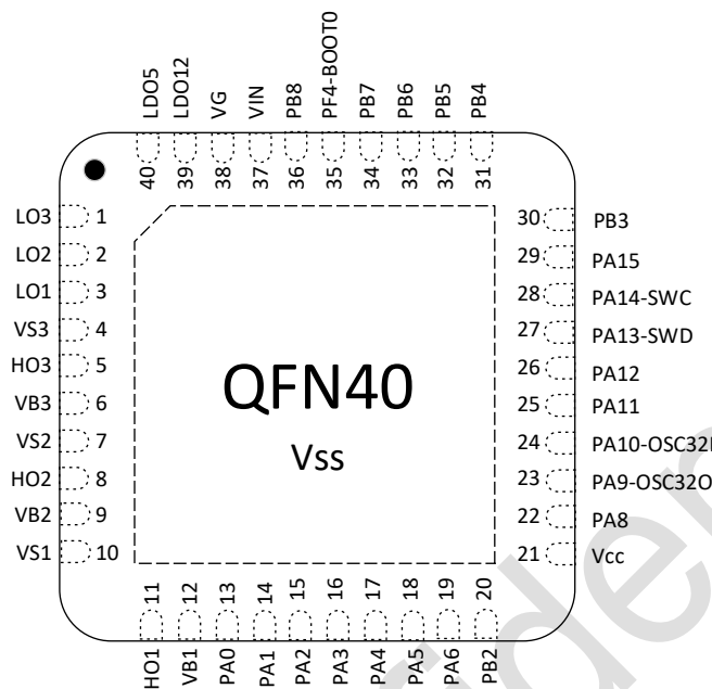
图 3-1 QFN40 Pinout2 PY32MD530H2xU7 (Top view)
